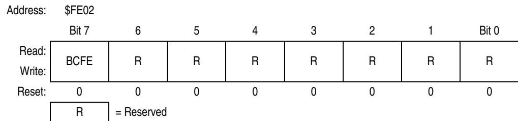
Figure 10-19. SIM Break Flag Control Register (SBFCR)
