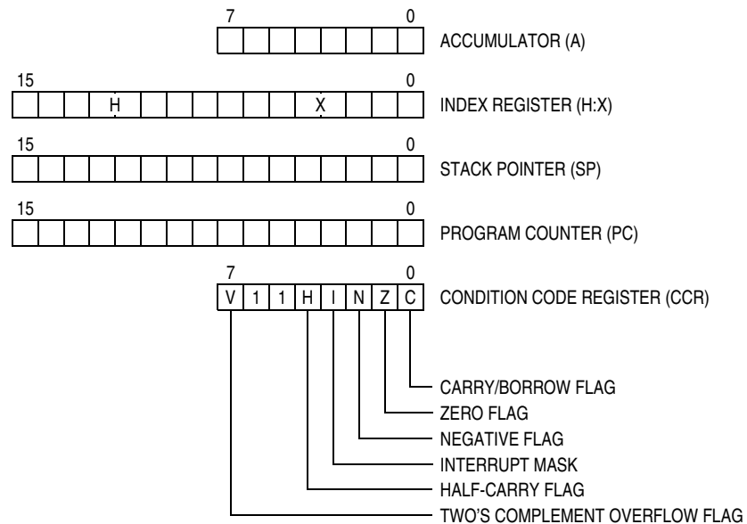
Figure 5-1. CPU Registers
